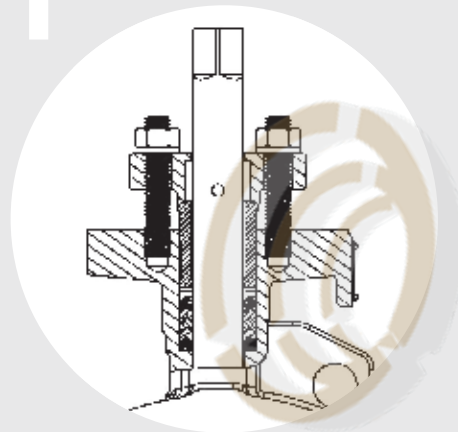
1 Standard V Type PTFE or RTFE Gland Packing System
