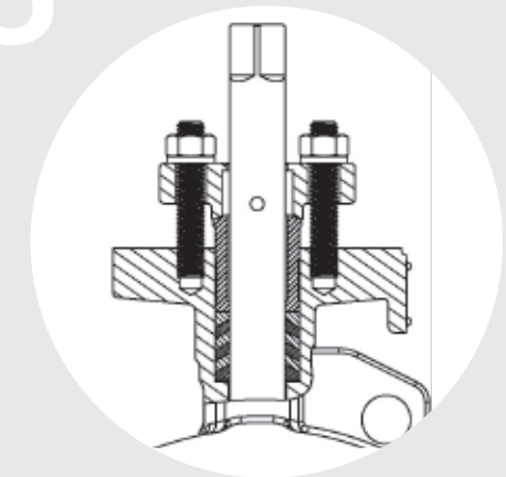
3 Standard GRAPHITE Packing System (Fire Safe Only)
